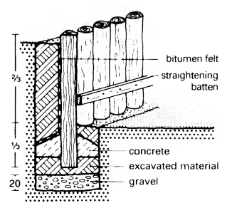
⑰ Wooden palisades
